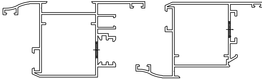
USINAGE 3.5
